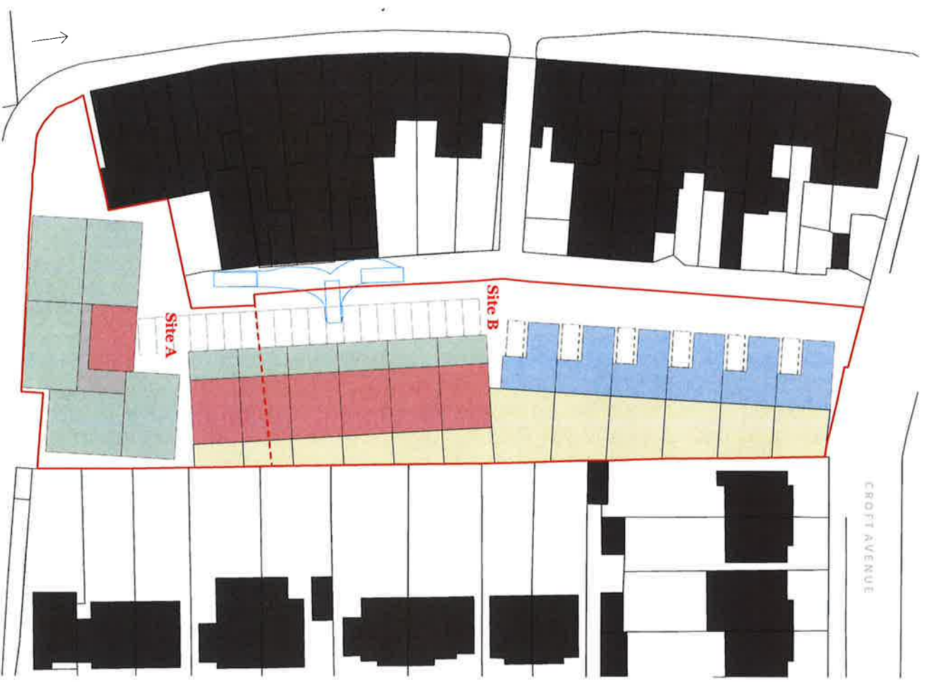
Site Plan 1:500 @ A3
